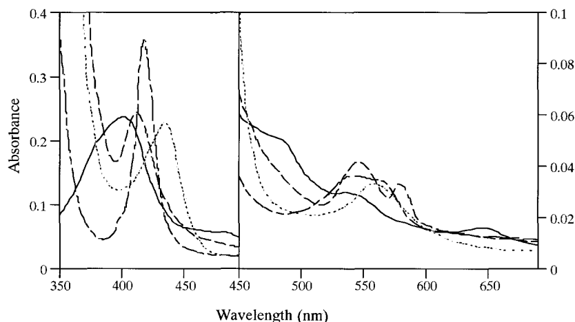
Fig. 2. Absorption spectra of the flavohemoglobin. Absorption spectra of FHb (0.8 \mu M in 50 mM sodium phosphate buffer (pH 7.2)) were measured at room temperature. Solid line, resting (oxidized); dotted line, dithionite-reduced; dashed line, NADH-reduced (1 mM NADH was added); dash-dotted line, dithionite-reduced plus CO.
