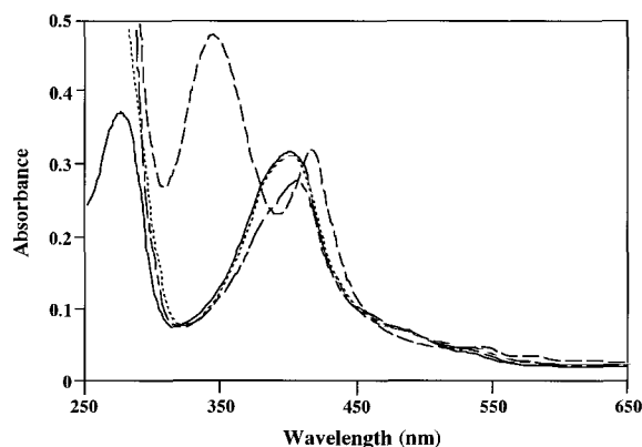
Fig. 3. Spectral changes of the flavohemoglobin upon incubation with NADH. FHb (0.8 \mu M) in 50 mM sodium phosphate buffer (pH 7.2) was mixed with 0.2 mM NADH under aerobic condition. Each spectrum shows: solid line, resting (oxidized); dashed line, at 10 s after addition; dash-dotted line, after 60 min; dotted line, after 300 min.
